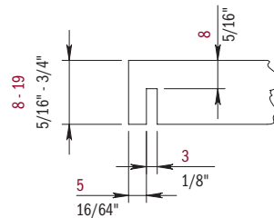
Machining for wood shelf
