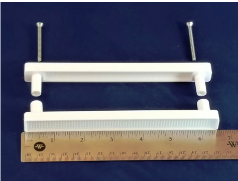
MagnaFold Handle Set, Inner, Outer, Screws PRT53
