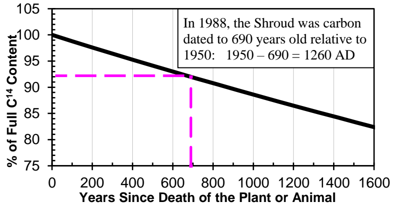
Figure 2. Amount C^{14} Decreases Due to Decay
