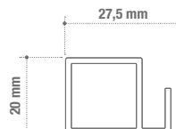
Front & rear 7713
