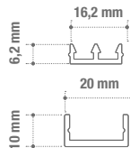
Sliding profile 7717+2362GV
