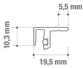
Upper rail 7715+CEP0037
