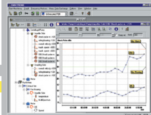
Evaluation of the data and archiving in the OMNITREND® database.
