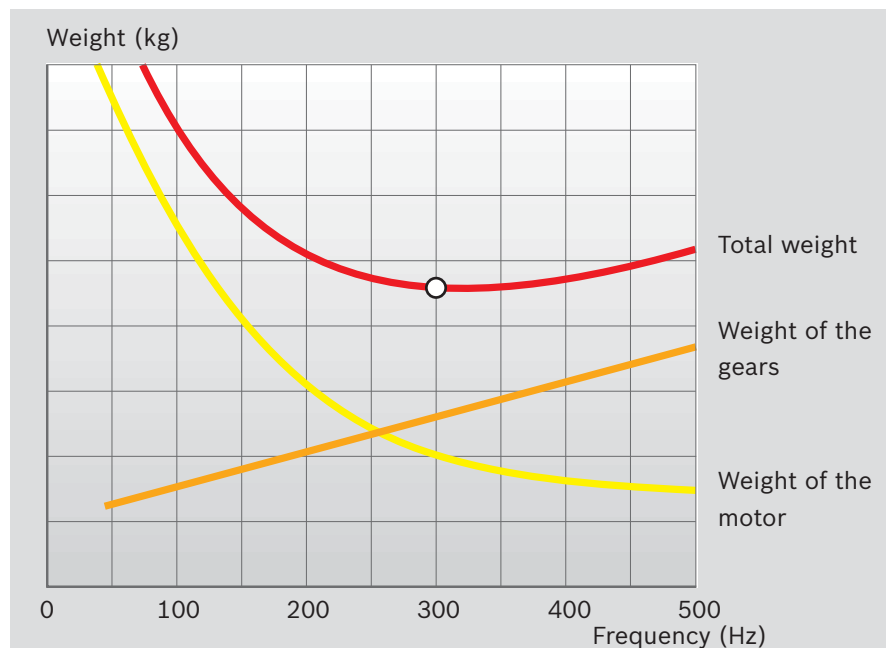
Fig. 1 The dependence of the motor and gear weight on the frequency at constant motor power and rated speed: The ratio of power to weight is optimal at 300 Hz.
