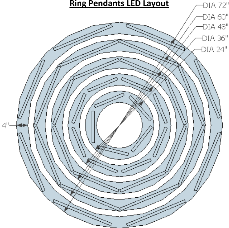
Ring Pendants LED Layout
