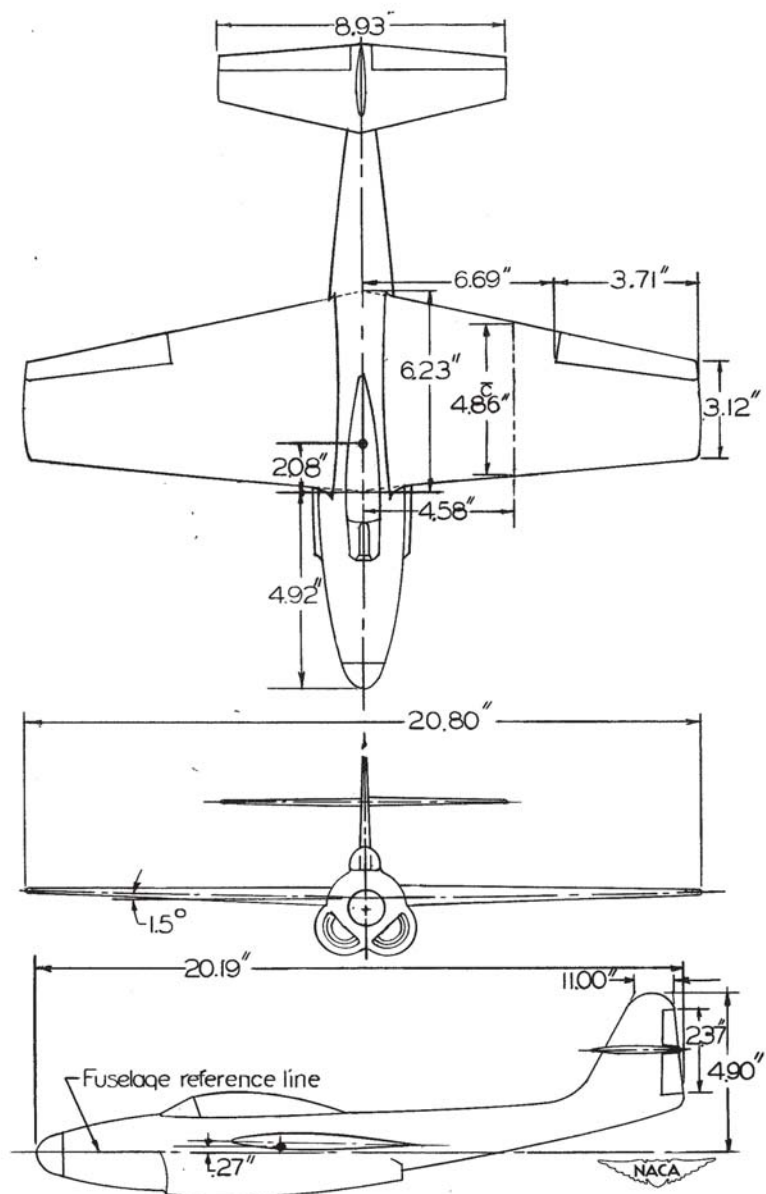
Figure 1. Three-view drawing of the Northrop XF-89 airplane. Dimensions are for 27-scale model
