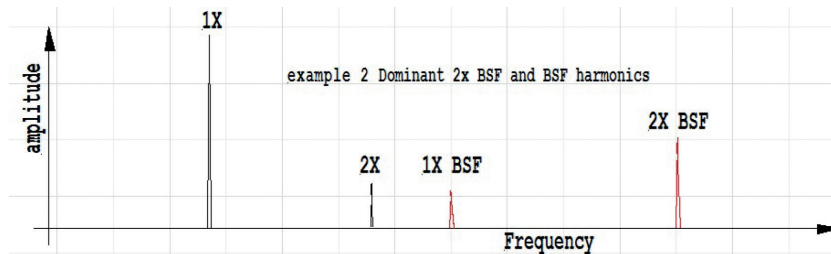
Dominant ball spin harmonics (2x BSF).
