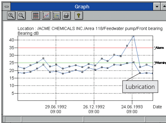
Typical shock pulse trend graph
