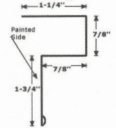
Overhang Trim
