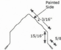
Small Corners/Rake
