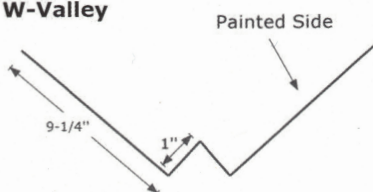
W-Valley
