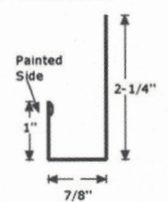
J-Channel
