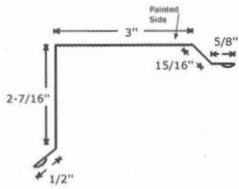
Residential Rake
