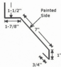
Track Cover
