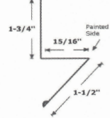
Rat Guard
