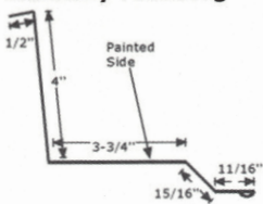
Chimney Flashing
