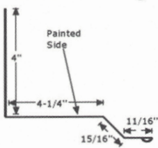
Sidewall Flashing
