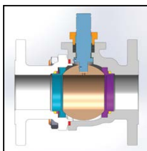
Scraper Design
