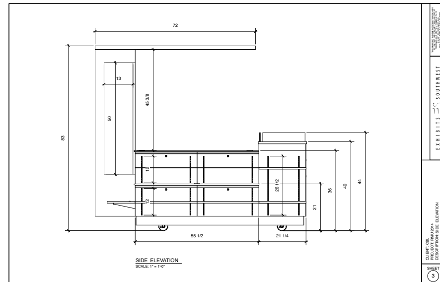
Model 2700 (plan & elevation)
