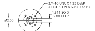
ACTUATOR SHOWN IN FULL CLOCKWISE POSITION FROM ACCESSORY SIDE.
