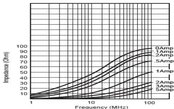
Impedance vs DC Bias BSM30 and BSM40
