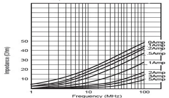
Impedance vs DC Bias BSM20
