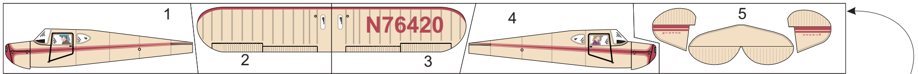
Placement of the individual panels on a 3"X36" sheet of 1/32" balsa
