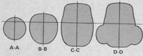
FUSELAGE CROSS-SECTIONS
