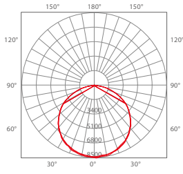
Lamp: 200W LED, 4000K, 125°
