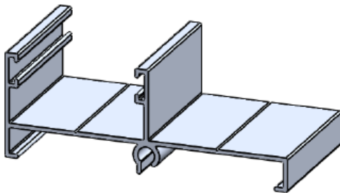
Horizontal Inf – EXA390
