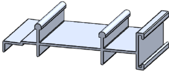
Sillar – EXA387
