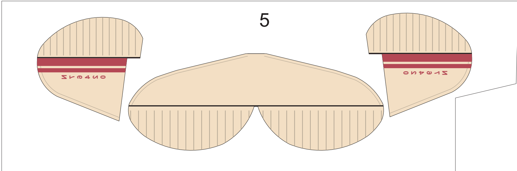
Placement of the individual panels on a 3"X36" sheet of 1/32" balsa
