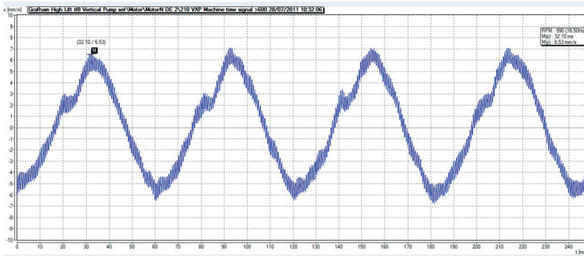
Time waveform of an unbalanced machine at 1000 rpm.
