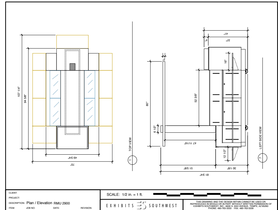
Model 2900 (plan & elevation)
