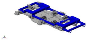
Project: Robotic Weld Fixture Notes: Fixture holds previously tack welded part for finish weld process via hydraulic swing clamps and work supports. Fixture utilizes spatter resistant materials, cable guards and sheet metal covers.
