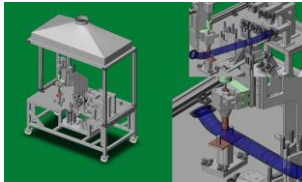
Project: Manual Sensor Boss Weld Station Notes: Station designed to adjust to twelve different exhaust pipe configurations. Table is height adjustable via hydraulic lift cylinders. Locating details utilize weld spatter resistant materials and coatings.
