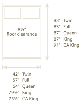
A CWF #1172 RAKE BED Headboard 54"h, Footboard 40"h
