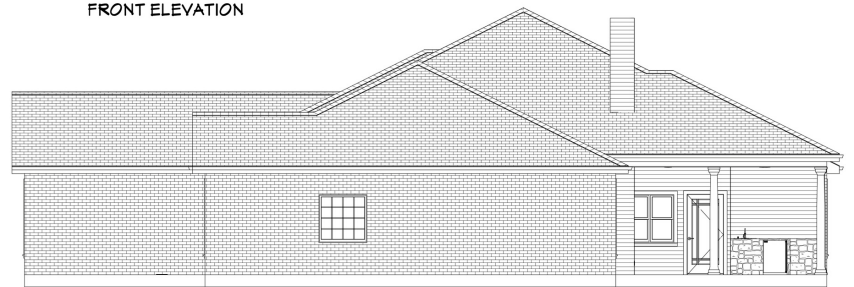
RIGHT SIDE ELEVATION
