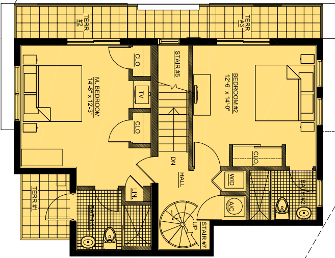
3RD FLOOR PLAN NOT TO SCALE
